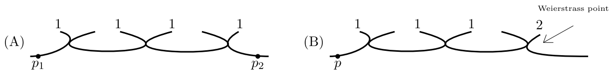
FIGURE 4. Curve (A) (respectively, (B)) is an elliptic (respectively, Weierstrass) chain of length 4.
