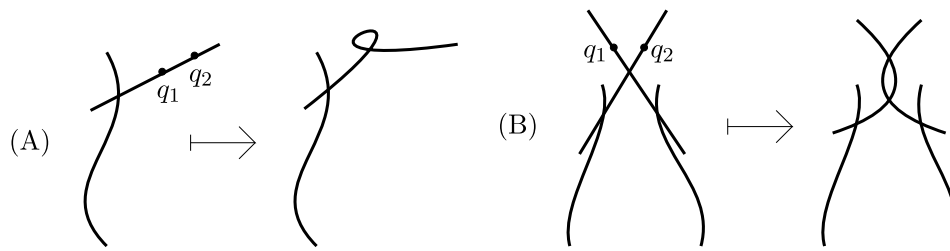
FIGURE 7. In (A), two marked points on a genus 0 tail (respectively, two conjugate points on an elliptic tail) are glued to yield an elliptic tail (respectively, a Weierstrass tail). In (B), two marked points on distinct rational components are glued to yield an elliptic bridge.
