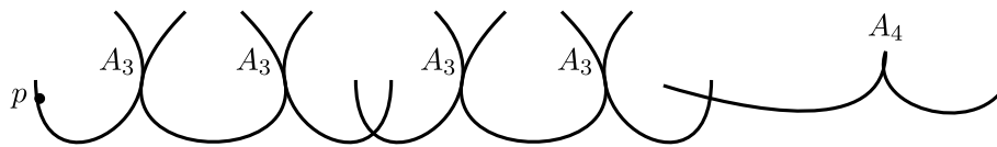
FIGURE 10. A \frac{2}{3} -link of length 3. Each component above is a rational curve.
