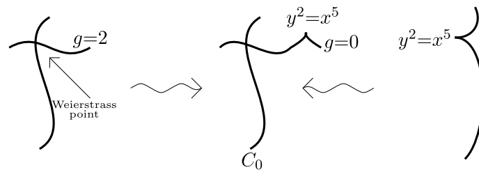
FIGURE 2. The curve C_0 is a nodal union of a genus g - 2 curve K and a rational ramphoid cuspidal tail. All curves obtained by either attaching a Weierstrass genus 2 tail to K at p , or imposing a ramphoid cusp on K at p , isotrivially specialize to C_0 . Observe that \text{Aut}(C_0) is not finite.
