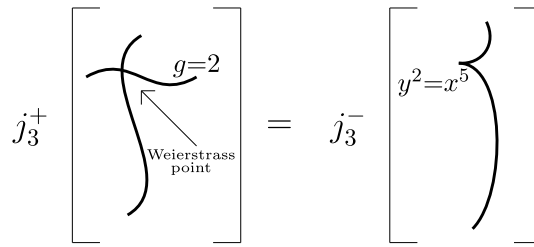
FIGURE 1. Curves with a nodally attached genus 2 Weierstrass tail are flipped to curves with a ramphoid cuspidal ( y^2 = x^5 ) singularity.
