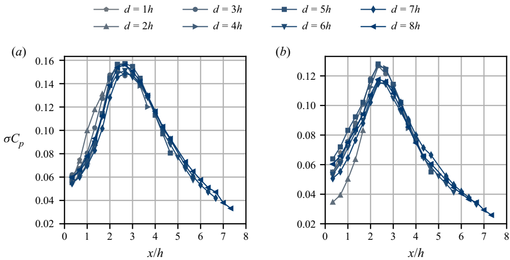
Figure 12. Standard deviation of pressure on the first-step floor with imposed forcing at St_h = 0.077 (a) and St_h = 0.149 (b).
