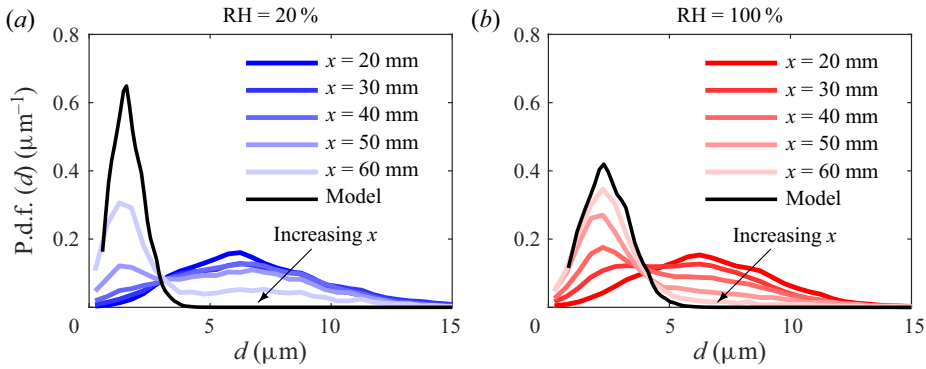
Figure 2. Droplet size distribution at (a) RH = 20% and (b) RH = 100% in a quiescent ambient environment. From dark to light, the line colour indicates an increasing distance x from the nozzle along the centreline, ranging from x = 20 to x = 60 mm. The solid black line is the predicted condensed water droplet size distribution based on the analytical model of Appendix A, valid for large distances x .
