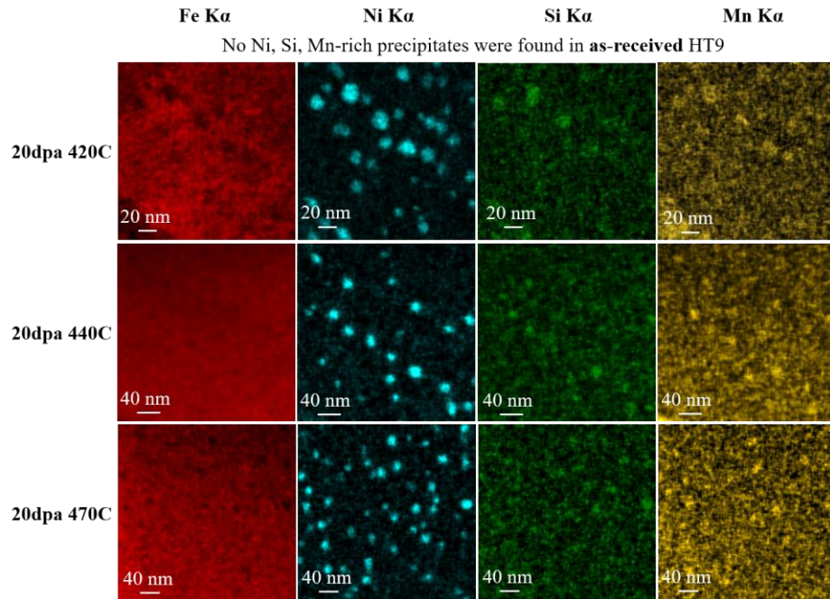
Figure 1. ChemiSTEM maps showed Ni, Si and Mn enrichment (associated with Fe depletion) in HT9 self-ion irradiated to 20 dpa at 420, 440 and 470°C. It indicates the formation of Ni, Si, Mn-rich precipitates in HT9 under irradiation.
