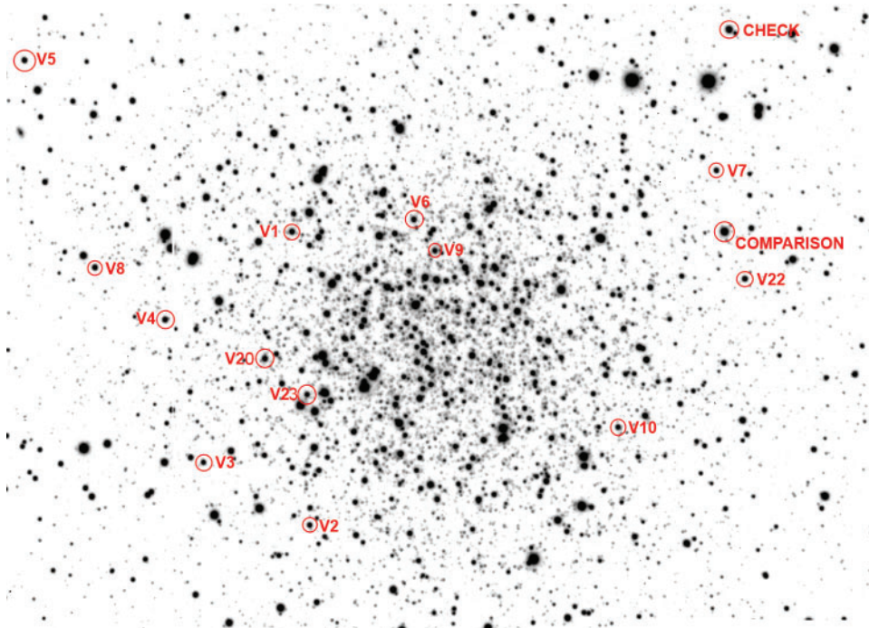
Figure 3 Finder chart constructed from V -band images used in this study. NE is at top left.
