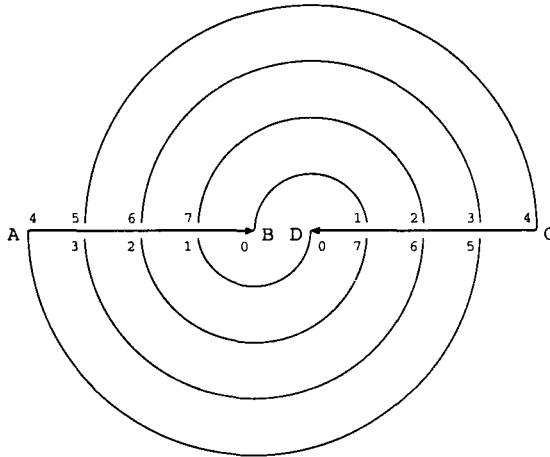
FIGURE 2. The two-component link K_{4,1} .
