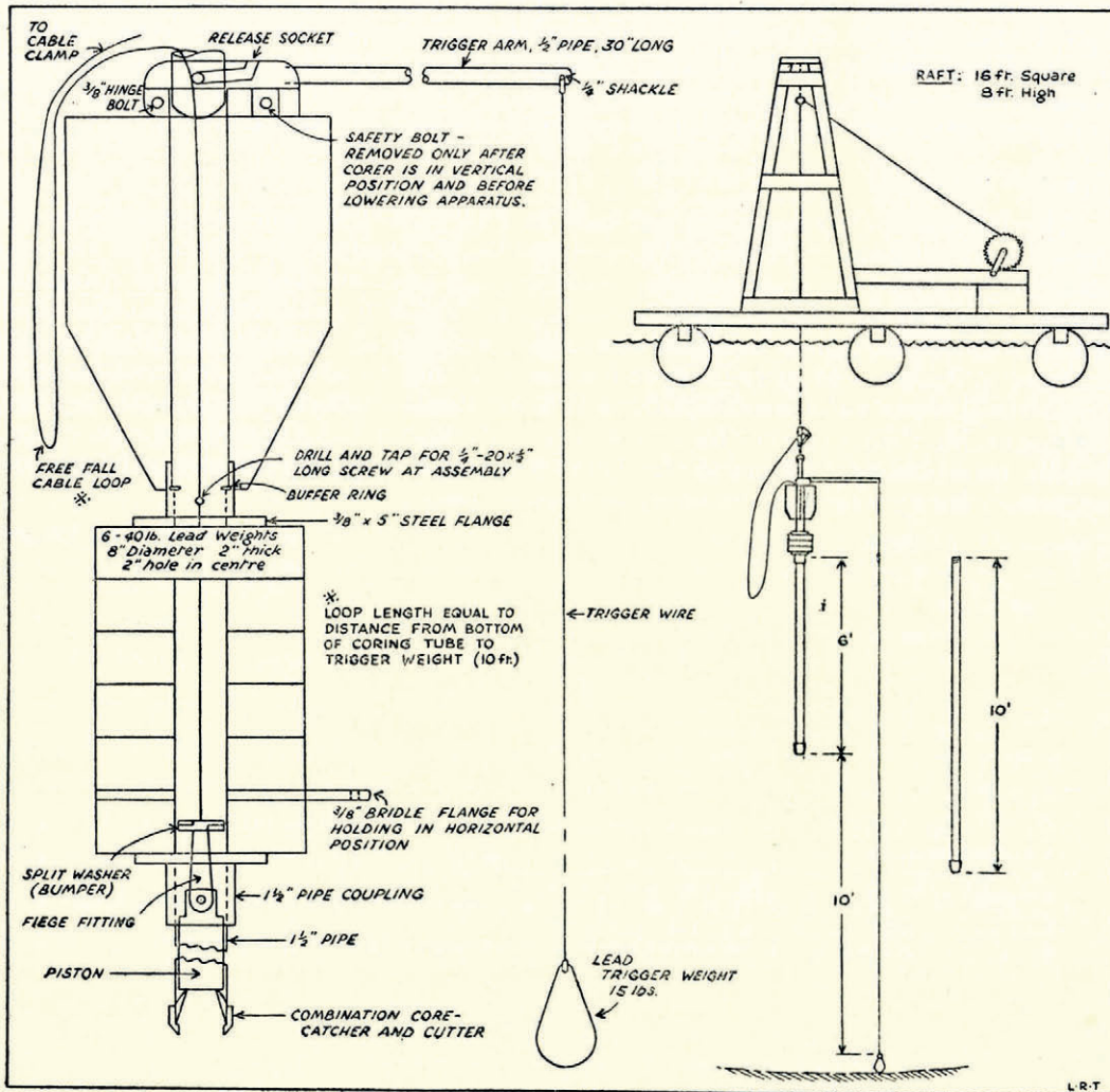
Fig. 1 (left). Detailed sketch of the instrumentation embodied in the piston-corer used for bottom sediment sampling of glacial lakes
