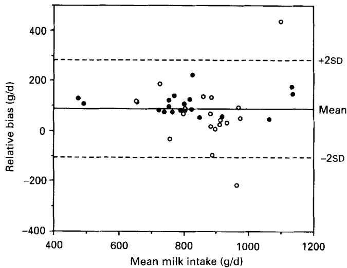
Fig. 1. Comparison between the deuterium dilution method, based on three biological half-lives of the isotope (3 t), and direct-weighing (DW) methods: relative bias plotted against the mean of the two methods. ●, Breast-fed infants; ○, formula-fed infants.
