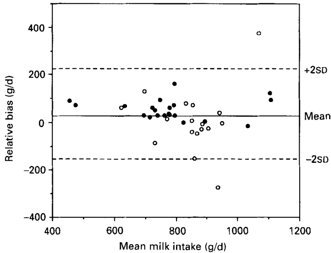
Fig. 2. Comparison between the deuterium dilution method, based on three biological half-lives of the isotope ( 3 t^{\frac{1}{2}} ) and corrected for environmental water influx, and direct-weighing (DW) methods: relative bias plotted against the mean of the two methods. ●, Breast-fed infants; ○, formula-fed infants.
