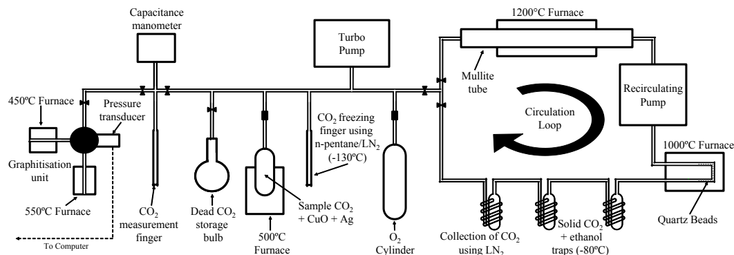
Figure 1 Vacuum system for extraction, purification, and graphitization of in situ-produced 14 C
