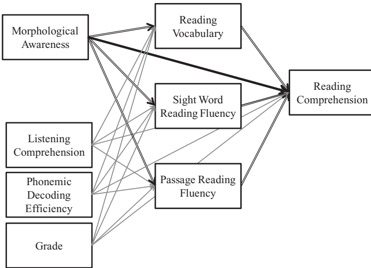
Figure 2. A path diagram representing the hypothesized path analysis model to address the second research question, with observed variables represented as rectangles, direct effect of interest represented as a black single-line arrow, moderated effects of interest represented as black double-line arrows, and effects of controls represented as gray arrows.
