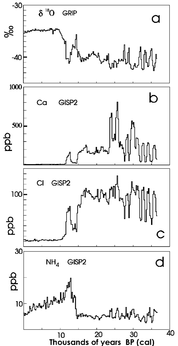
Fig. 2. Summit ice-core records: (a) \delta^{18}\text{O} from the GRIP core (Johnsen and others, 1997); (b) \text{Ca}^{2+} concentration (ppb) (mass) in GISP2 core (Mayewski and others, 1997); (c) \text{Cl}^- concentration (ppb) in GISP2 ice core; (d) \text{NH}_4^+ concentration (ppb) in GISP2 core.
