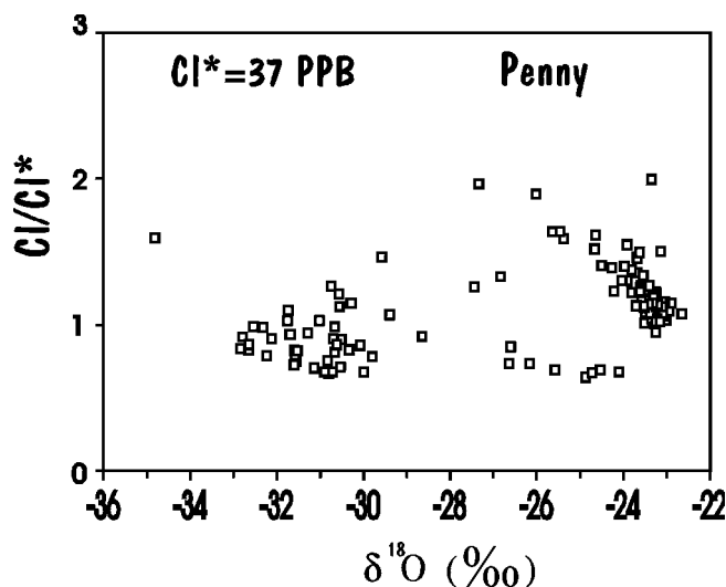
Fig. 7. Penny Ice Cap chlorine vs uncorrected \delta^{18}\text{O} for early-Holocene and ice-age ice. The early-Holocene \delta^{18}\text{O} values have probably been affected by meltwater from the wasting Laurentide ice cap and consequently need correcting. For corrected version of this figure see Figure 8b.
