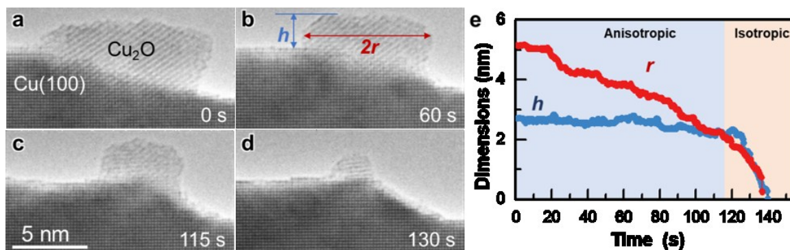
Figure 2. Figure 2. In situ ETEM reduction of \text{Cu}_2\text{O} island grown on \text{Cu}(100) surface under 0.1 Pa MeOH at 300 °C. (a-d) Atomic resolution HRTEM images of the reduction process. (e) Plot of radius ( r , red, half of the width) and height ( h , blue) of the \text{Cu}_2\text{O} island as a function of time, in which two-stage reduction can be observed.
