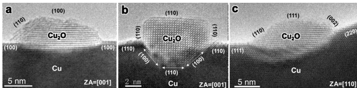
Figure 1. Figure 1. HRTEM images of \text{Cu}_2\text{O} islands grown on different Cu substrate orientations via in situ oxidation. (a) \text{Cu}_2\text{O} island grown on \text{Cu}(100) facet. (b) \text{Cu}_2\text{O} island grown on \text{Cu}(110) facet. (c) \text{Cu}_2\text{O} island grown on \text{Cu}(111) facet.
