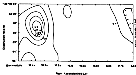
Figure 6. Detailed distribution of \text{H}_2\text{O} maser components in Sgr B2 (M), superimposed on the 5 GHz continuum map. The contour levels are at 29 \times (2, 3, 4, 5, 6, 7) mJy per beam. The beam size is 2.7'' \times 1.6'' at P.A. = 11^\circ.7 . The positions of maser spots are indicated by the dots.
