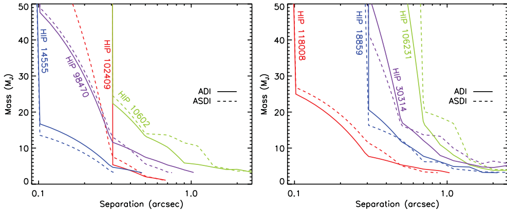
Figure 2. Sensitivity limits at 5\sigma of the survey in Jupiter masses of detectable companions (BT-Settl models, Allard et al. 2011) for the youngest stars of the survey ( \leq 70 Myr). The curves are derived for two pipelines: classical ADI (solid curves) and ASDI (dashed curves).
