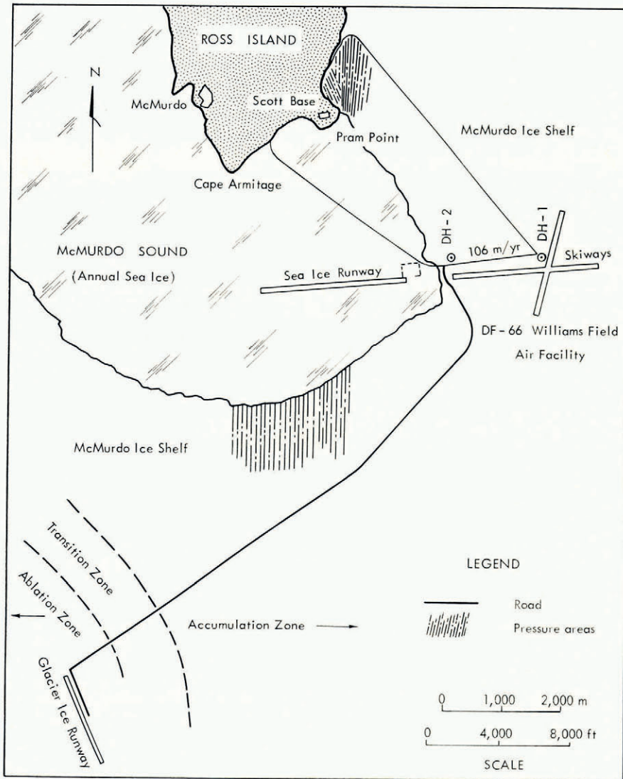
Fig. 1. Sketch map of the area between McMurdo station and "Outer Williams Field", McMurdo Sound, Victoria Land, Antarctica.
