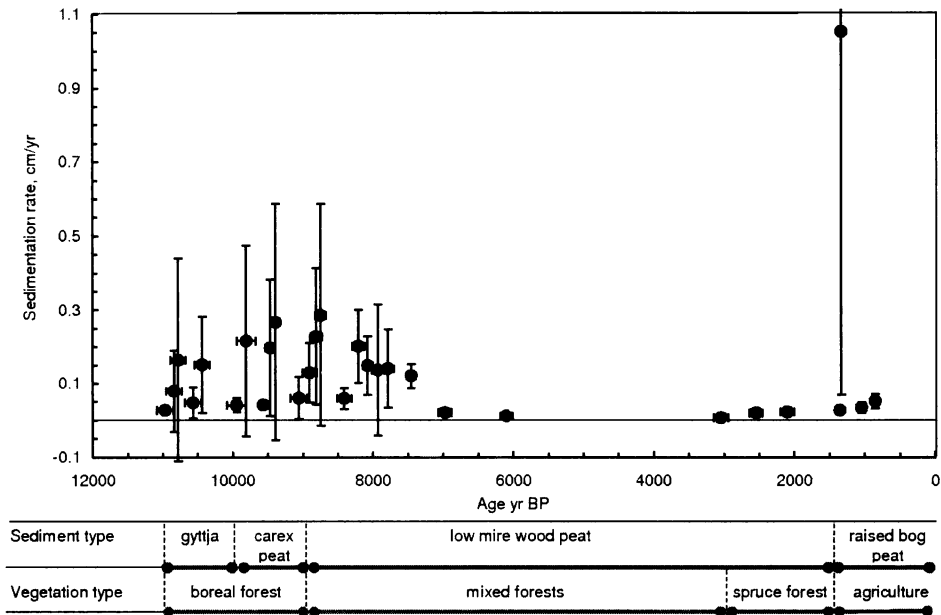
Figure 3 Sedimentation rate, as a function of time, for the NO raised peat bog. The lower part of the figure indicates the sediment vegetation types (the latter based on pollen analysis as described in the text).
