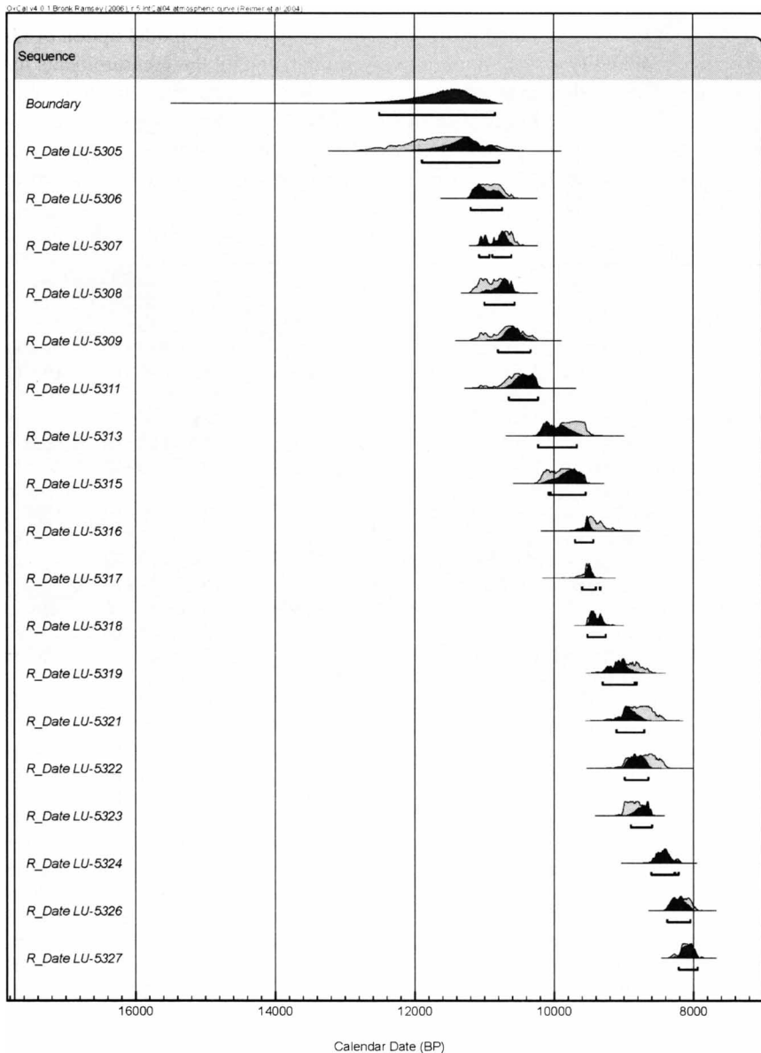
Figure 2 OxCal Sequence deposition model option for NO raised peat bog
