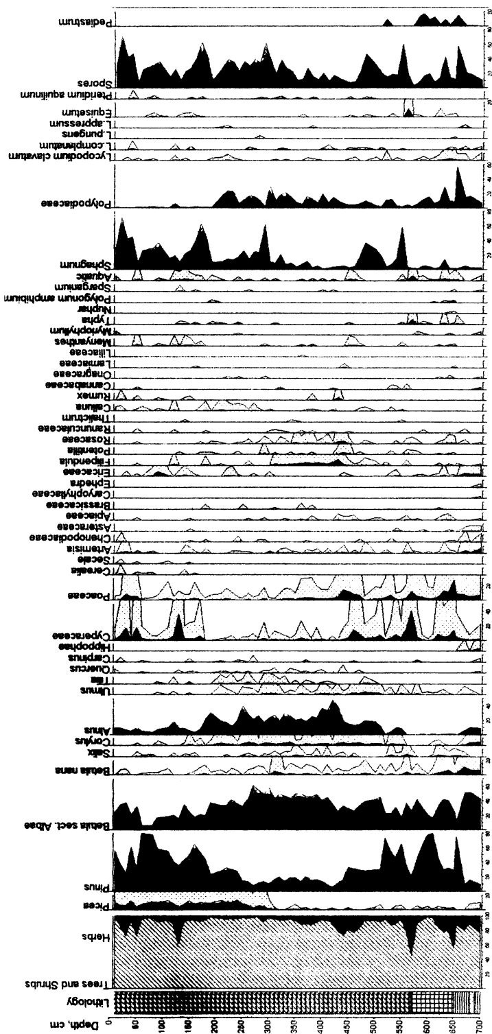
Figure 4 Pollen diagram for NO raised peat bog (analysis by L. A. Savileva in 2005)
