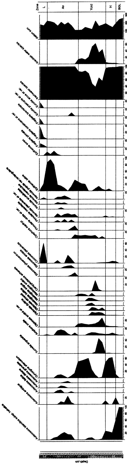
Figure 5 Diatom diagram for NO raised peat bog
