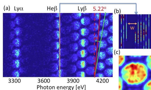
Figure 3. (a) MMI data with an inappropriate PHA tilt. The dashed line is the reference vertical line (i.e., \theta = 0^\circ ). The red and green solid lines show the extracted ( 5.22^\circ ) and optimal ( 8.95^\circ ) PHA tilt angles. (b) Monochromatic image reconstructed from a single pixel column at the He- \beta line center. (c) Narrow-band He- \beta image reconstructed over its linewidth (i.e., \sim 60 eV).
