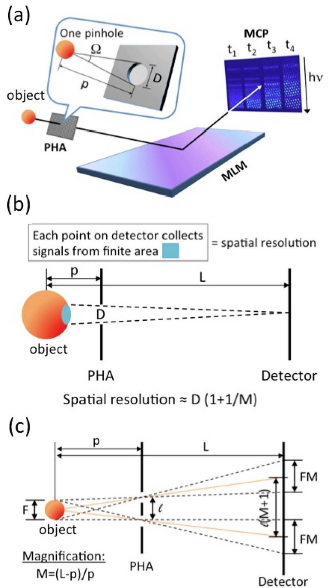
Figure 1. (a) The MMI consists of a PHA, a MLM and a MCP. The signal collected through a pinhole is proportional to the source-to-pinhole solid angle, \Omega = \pi D^2/4p^2 . (b) The spatial resolution is determined by the object–pinhole–detector distances. (c) The magnification is determined by the object–pinhole distance, p , and the object–detector distance, L . The optimal pinhole separation, l , is determined so that images of size FM do not overlap.
