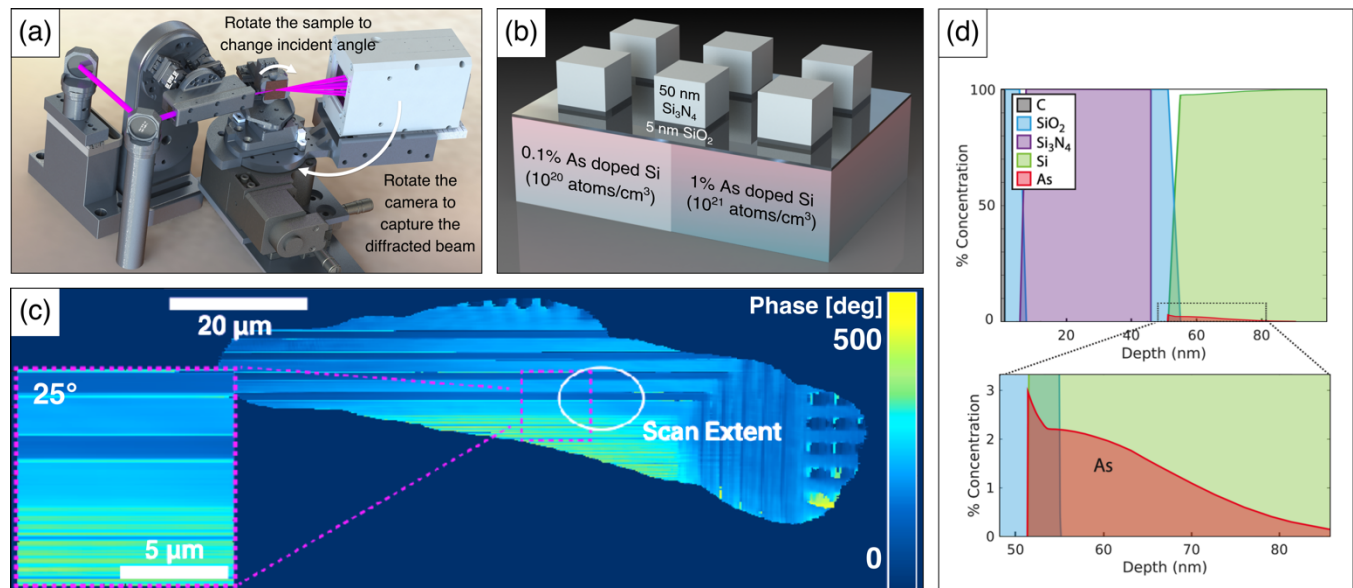
Figure 1. EUV complex imaging reflectometry experiment. (a) The experimental setup schematic. (b) The sample, with Si 3 N 4 /SiO 2 structures atop Si substrate, with spatially varying degrees of As doping. (c) Ptychographic phase image of the sample at 25° from grazing; inset showing the high-fidelity region near the scan extent. (d) Reconstructed depth-dependent chemical composition of a structure on a highly doped region.
