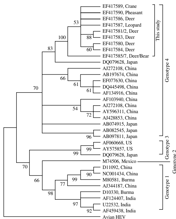
Fig. 2. Phylogenetic tree constructed by alignment of the 299-nt nucleotide sequence of ORF2 from isolates in this study and 26 references of other animal and human HEV isolates, using the neighbour-joining method and evaluated using the interior branch test method with Mega2.0 software. Percent bootstrap support is indicated at each node. An avian HEV strain is included as outgroup.
