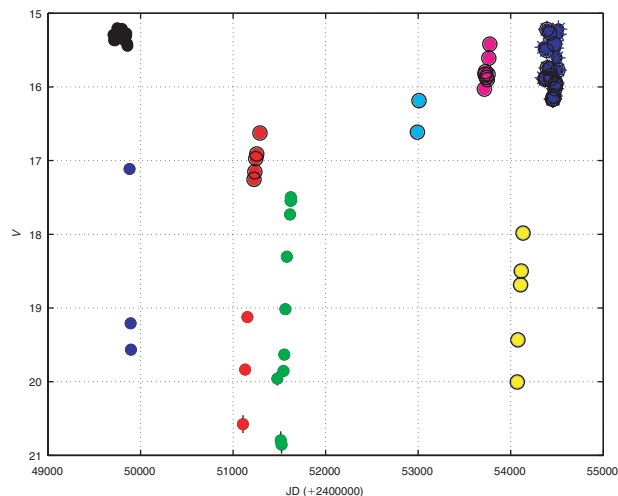
Figure 2 The light curve ( V ) for LMC100.6 48589 displaying the seven declines (separately colour-coded) in the time interval of this research. The solid black points are data obtained at maximum light, while the black circled points are the data selected for use in further decline recovery calculations.
