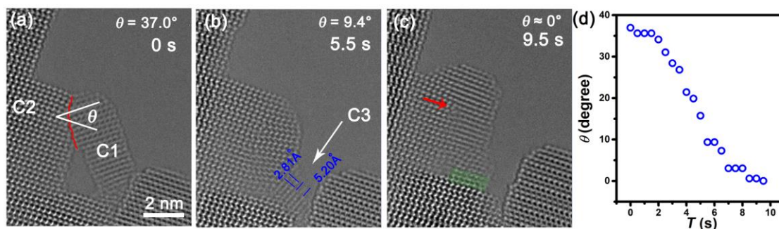
Figure 2. Coalescence of two ZnO crystals. (a) HRTEM image showing the angle \theta between the (0002) planes of Crystal 1 (C1) and Crystal 2 (C2). (b) The rotation of C1 resulting in the decrease of \theta . The newly formed Crystal 3 (C3) are indicated by the arrow. (c) The rotation of C3. (d) The relationship between \theta and the irradiation time T .
