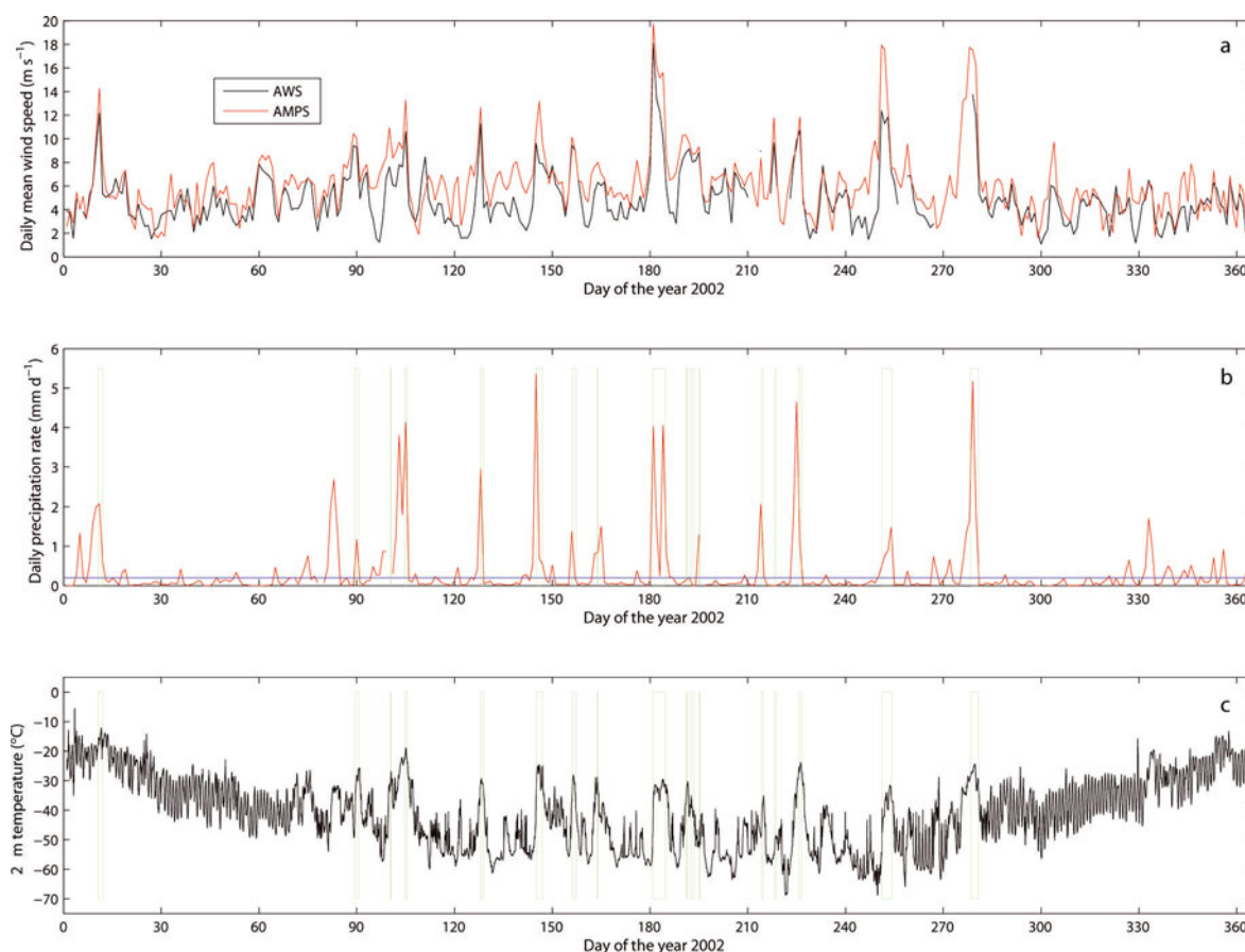
Fig. 6. (a) Time series of daily mean wind speed derived from AWS9 data (black) and AMPS forecast data (red) for 2002. (b) Time series of daily precipitation rate derived from AMPS forecast data (red) for 2002. Periods of strong-wind events identified on the basis of 2 hour mean values of wind speed measured at AWS9 are indicated by green rectangles. The blue line indicates a daily precipitation rate of 0.2 \text{ mm w.e. d}^{-1} . (c) Time series of 2 hour mean temperature at 2 m height at AWS9 (black) for 2002. Periods of strong-wind events identified on the basis of 2 hour mean values of wind speed measured at AWS9 are indicated by green rectangles.
