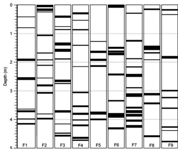
Fig. 4. Dune horizons (black horizontal bars of different thickness) in nine firn cores (F1–F9) covering a time interval of 22 \pm 2 years. The cores were drilled along a 600 m long traverse route. The number of dune layers varies between 6 and 12.
