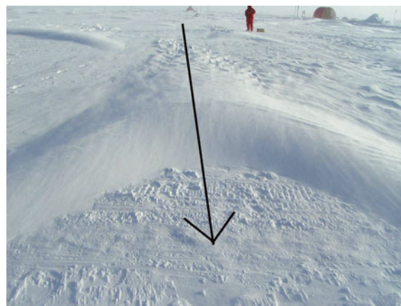
Fig. 2. Newly formed barchan-type snow dune at Kohnen station on 28 January 2006. The arrow indicates the near-surface wind direction.
