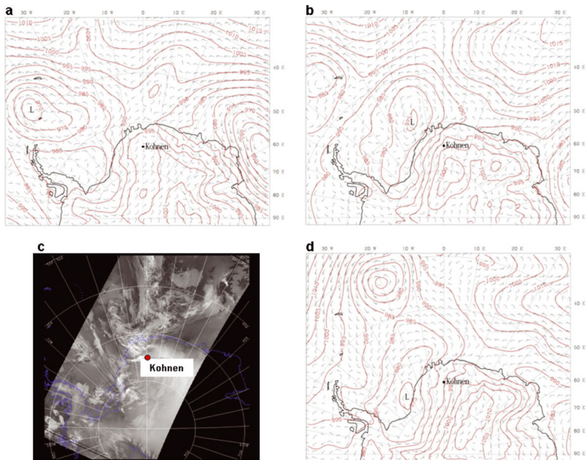
Fig. 9. (a, b, d) Sea-level pressure and near-surface horizontal wind vectors (full barb indicates 5 \text{ m s}^{-1} ) provided by AMPS analysis at 0000 UTC: (a) on 9 January 2006, (b) on 11 January 2006 and (d) on 12 January 2006. The black letter L indicates the center of a low-pressure system. (c) AVHRR satellite image in the infrared range on 11 January 2006, 0309 UTC. The coastline of Antarctica and the inner boundary of the ice shelves are indicated in blue.
