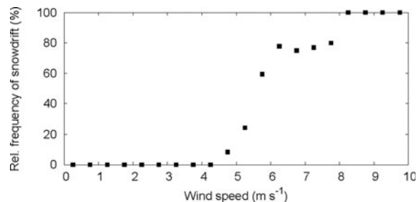
Fig. 5. Relative frequency of observed snowdrift as function of 1 hour mean wind speed at 2 m height at AWS9 in the 2005/06 austral summer.
