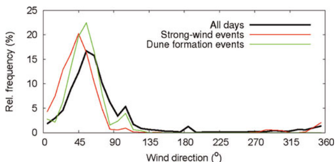
Fig. 7. Relative frequency of 2 hour mean wind direction at 2 m height at AWS9 in the whole period 1998–2000/2002–05 (black curve), during all strong-wind events (red curve) and during all barchan-type dune formation events (green curve).
