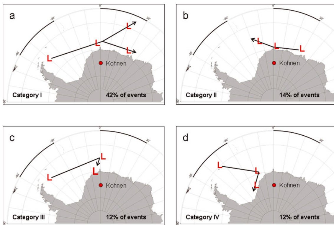
Fig. 8. Synoptic developments causing strong-wind events at Kohnen station: pattern for category I (a), category II (b), category III (c) and category IV (d). The red character L indicates the center of a low-pressure system. The black straight lines and arrows show the track of a low-pressure system in a simplified way.
