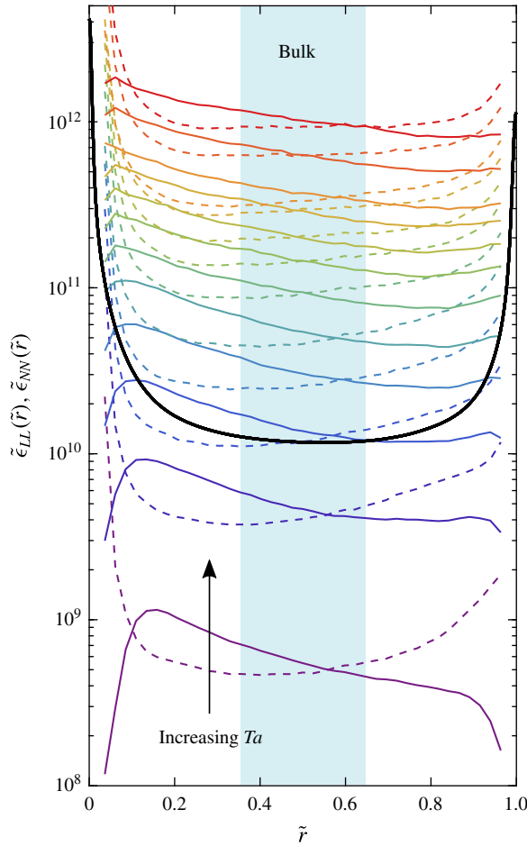
FIGURE 3. (Colour online) Dimensionless energy dissipation rate profile \tilde{\epsilon}(r) = \epsilon(r)/(d^{-4}v^3) for various Ta : longitudinal direction \tilde{\epsilon}_{LL}(\tilde{r}) (dashed lines), transversal direction \tilde{\epsilon}_{NN}(\tilde{r}) (solid lines). Ta is increasing from bottom to top, the lines correspond to the following Ta numbers: Ta = 4.0 \times 10^8 , 1.6 \times 10^9 , 3.6 \times 10^9 , 6.4 \times 10^9 , 1.0 \times 10^{10} , 1.4 \times 10^{10} , 2.0 \times 10^{10} , 2.6 \times 10^{10} , 3.2 \times 10^{10} , 4.0 \times 10^{10} , 5.7 \times 10^{10} , 9.0 \times 10^{10} . For every Ta , both \epsilon -profiles cross within the bulk region ( \tilde{r} \in [0.35, 0.65] ) which is highlighted in blue. The black solid line is the total energy dissipation rate obtained from DNS for Ta = 2.15 \times 10^9 (Zhu, Verzicco & Lohse 2017).
