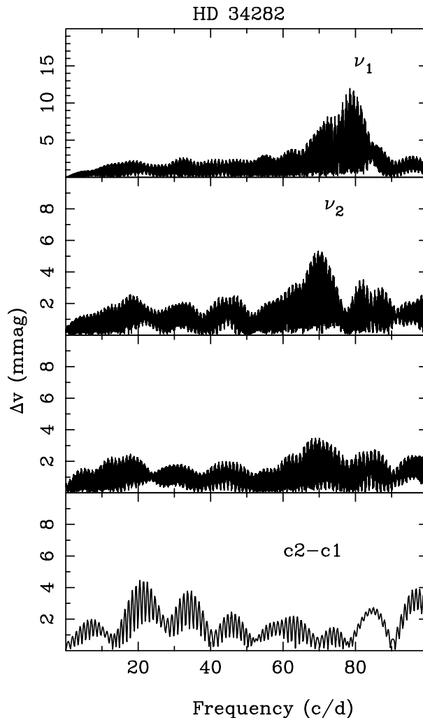
Figure 3. Fourier analysis of the Strömgen v data. The Fourier transform of the differential photometry of the comparison stars (C2–C1) is given in the bottom panel.
