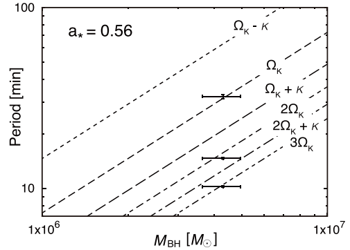
Figure 2. Observed QPOs of Sgr A* as a function of its mass. Lines show \Omega_K - \kappa , \Omega_K , \Omega_K + \kappa , 2\Omega_K , 2\Omega_K + \kappa and 3\Omega_K , which are expected with the resonant disk oscillation model (Kato et al. 2010).
