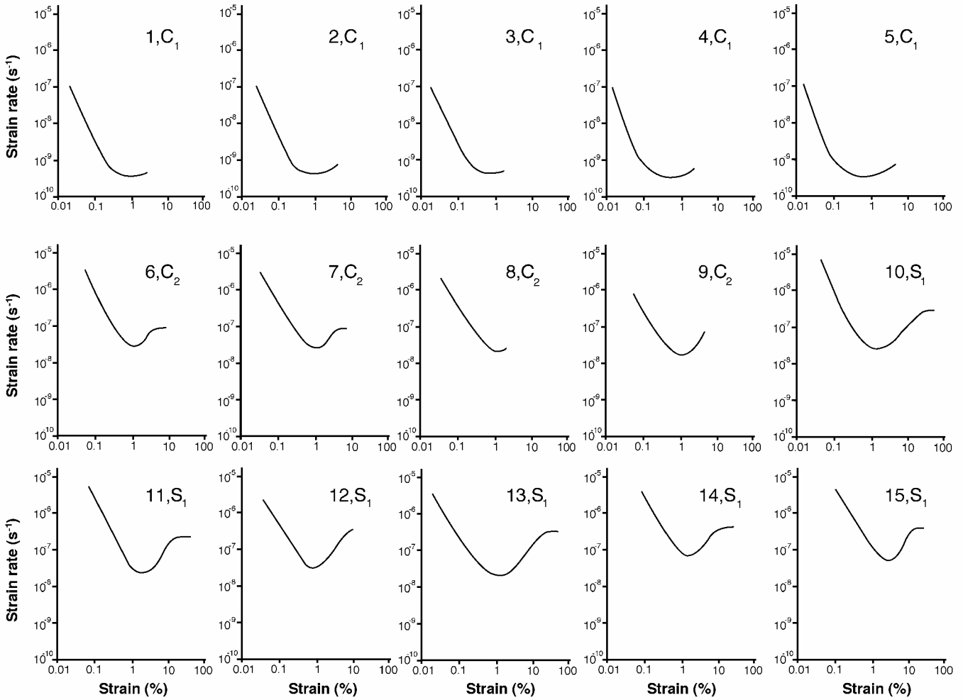
Fig. 1. Creep curves (plots of octahedral strain rate as a function of octahedral strain) for each of the tests in compression (labelled C_1 and C_2 ) and shear (labelled S_1 ) under constant load. Temperature, stress, debris content and other details are provided in Table 1.
