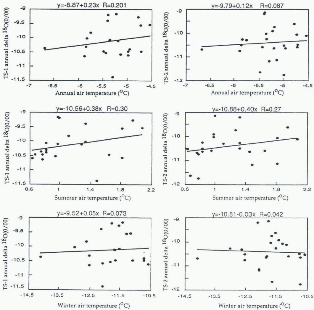
Fig. 5. The linear relationship between annually averaged \delta^{18}O and contemporaneous annual, summer and winter surface temperature.
