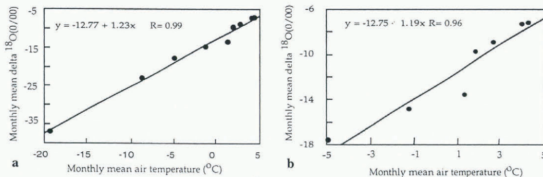
Fig. 3. The linear relationship between monthly-averaged \delta^{18}\text{O} and monthly-averaged air temperature T_a : (a) annual; (b) summer. Both are significant at p = 0.001 . No precipitation samples were collected during November–December 1995 and February–March 1996.
