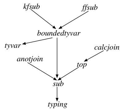
Fig. 6. Subtyping features
