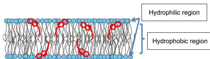
Fig. 1. \alpha -Tocopherol localisation in a membrane lipid bilayer.
