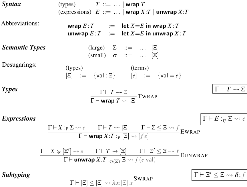
Fig. 9. Extending IML ex with impredicativity.
