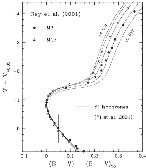
Figure 2. The fiducial sequence for M3 is compared with that for M13 following the prescription of Vandenberg et al. (1990). Note the separation between the two clusters' RGBs, indicating an age difference.
