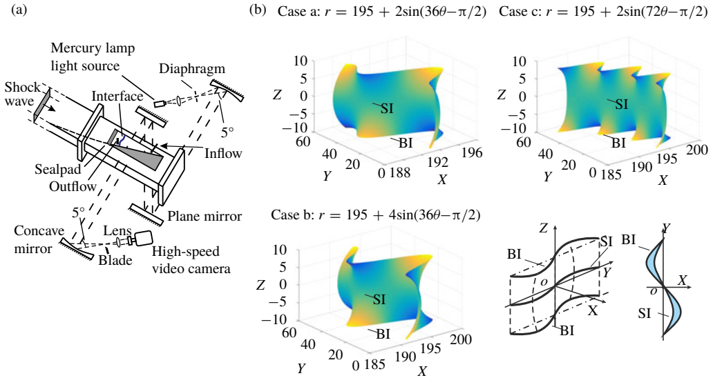
FIGURE 2. (Colour online) Schematic of schlieren photography system (a), and the three sinusoidal interfaces with a sketch of the minimum surface feature and a top view of the interface (b). BI: boundary interface, SI: symmetry interface.
