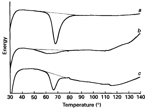
Fig. 4. Differential scanning calorimetry traces for (a) raw green-banana flour, (b) a pooled ileal sample containing undigested banana starch, and (c) a resistant starch residue prepared in vitro from green-banana flour.
