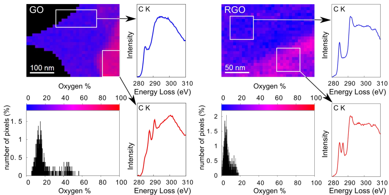
Figure.1 Chemical maps of GO and RGO flakes and related histogram of oxygen occurrence. Carbon K-edges fine structures extracted from the marked regions in the maps.
