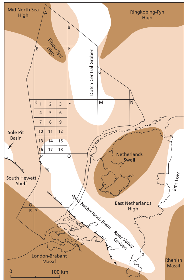
Fig. 3. Map of latest Triassic to Middle Jurassic structural elements (after Van Adrichem Boogaert & Kouwe, 1993; Wong, 2007). Dark brown colour: structural high, partly subaerial landmass; light brown colour: platform, intermittently flooded; white: basin.
