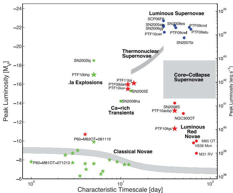
Figure 1. Framework of Cosmic Explosions expressed as peak luminosity versus characteristic time-scale. In 2005 we only knew about classical novæ and supernovæ (grey bands). In the past 5 years systematic searches, serendipitous discoveries and archival searches have uncovered a plethora of novel, rare transients. Several new classes are emerging, and the governing physics is being widely debated: luminous red novæ (the electron-capture induced collapse of rapidly rotating O–Ne–Mg white dwarfs?), luminous supernovæ (magnetars or pair instability explosions?), Type Ia explosions (helium detonations in ultra-compact white-dwarf binaries), calcium-rich halo transients (helium deflagrations or fallback onto a black hole?) (from Kasliwal, M.M., 2011, PhD Thesis, California Institute of Technology).
