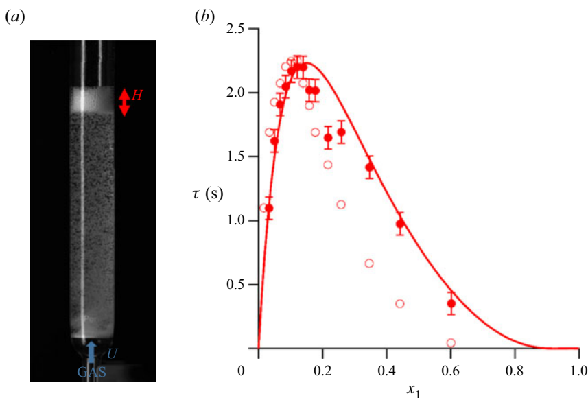
Figure 3. (a) Foam of stationary height H formed by continuous injection of gas at velocity U in a Bikerman column filled with a decane-toluene mixture. (b) Lifetime of the foam, as defined by (3.1), as a function of the molar fraction in decane. The experiment was performed in an open column (open circles) and in closed gas circulation (full symbols). The full line is a guide for the eye. For the sake of clarity, error bars (corresponding to the uncertainty on foam height) are shown for only one set of data.
