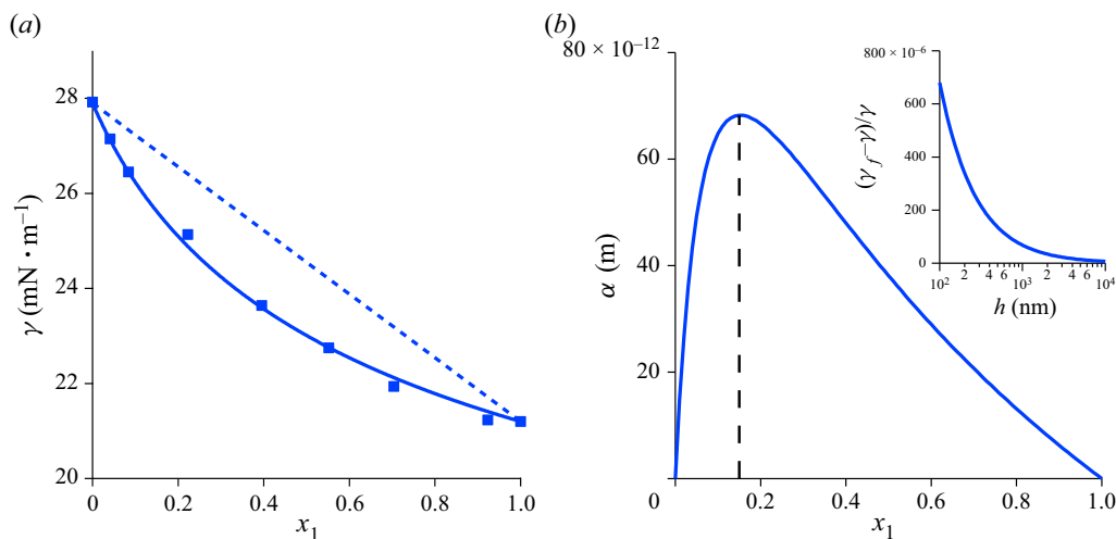
Figure 2. (a) Surface tension of a mixture of octane and toluene as a function of the molar fraction in octane. The full line is an interpolation of the experimental data (symbols). The dotted line indicates linear behaviour. (b) Corresponding variations with composition of length \alpha computed from (2.4) with v = 1.64 \times 10^{-4} \text{ m}^3 \text{ mol}^{-1} and \sigma = 0.25 \times 10^6 \text{ m}^2 \text{ mol}^{-1} . The relative variation of the thickness-dependent surface tension of a film of thickness h computed from (2.2) is shown in the inset for the maximum value of \alpha indicated by the dashed line.
