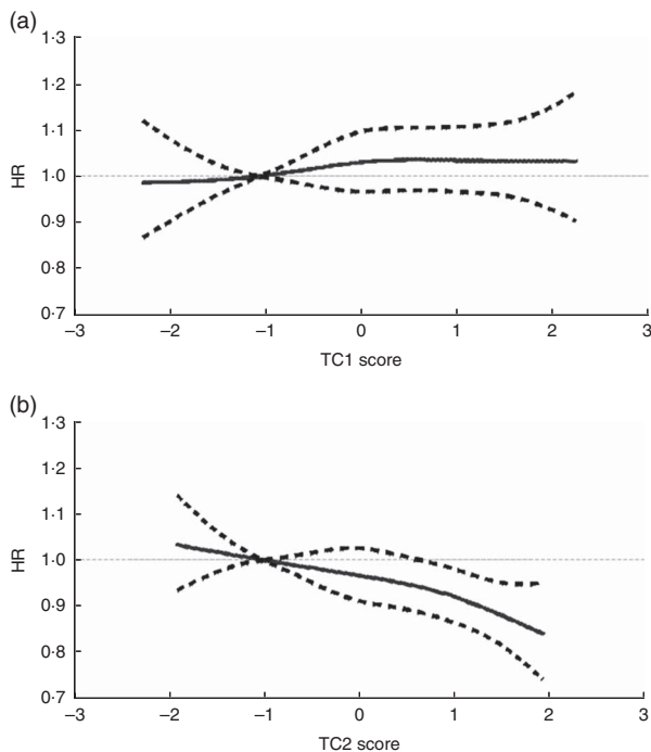
Fig. 2 Relationship between nutrient patterns derived from treelet transform and breast cancer risk (—, hazard ratio (HR); - - - -, associated 95% CI), obtained by using restrictive cubic splines with values of 1st and 99th percentiles and medians of quintiles 1, 3 and 5 used as knots, among 334 850 women in the European Prospective Investigation into Cancer and Nutrition (EPIC): (a) first treelet component (TC1), P_{\text{non-linearity}}=0.94 , P_{\text{trend}}=0.88 ; (b) second treelet component (TC2), P_{\text{non-linearity}}=0.77 , P_{\text{trend}}=0.02 . Models were stratified by study centre and age in 1-year categories and adjusted for baseline menopausal status (premenopausal and perimenopausal (reference) or postmenopausal and women who underwent an ovariectomy), baseline alcohol intake (never drinkers (reference), former drinkers, drinkers only at recruitment, lifetime drinkers, unknown), height (continuous), BMI (below (reference) or above 25 kg/m 2 ), schooling level (none, primary (reference), technical/professional/secondary, longer education, unknown/unspecified), age at first full-term pregnancy (nulliparous (reference), \leq 21 years, 21–30 years, >30 years, unknown or missing), age at menarche ( \leq 12 years (reference), 12–14 years, >14 years, missing), age at menopause ( \leq 50 years (reference), >50 years, pre-menopause or missing), use of hormone replacement therapy (never (reference), ever, unknown), level of physical activity (inactive (reference), moderately inactive, moderately active, active, unknown) and alcohol-free energy (continuous). P_{\text{trend}} was obtained by evaluating the joint significance of variables other than the linear one in the model by using Wald's test with df=3
