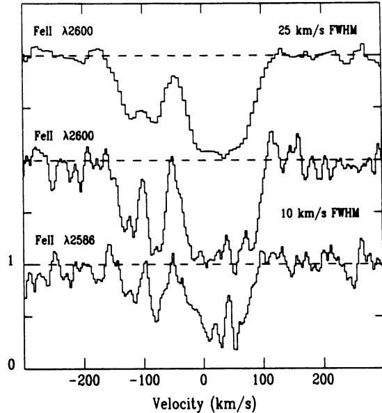
Figure 1. Fe II at z = 1.345 .
