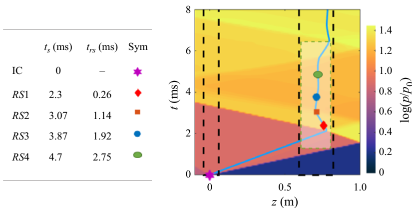
Figure 2. Experimental z - t diagram with window locations shown with dashed black lines, the interface location in blue and HS PLIF FOV shown as the highlighted rectangle. Individual symbols refer to single-shot (SS) times. Here, t = 0 and z = 0 refer to the time and space location of the initial shock–interface interaction; t_s denotes the time after shock and t_{rs} is the time after reshock; RS1 – 4 are the labels for the four post reshock times investigated in the SS experiment campaign.
