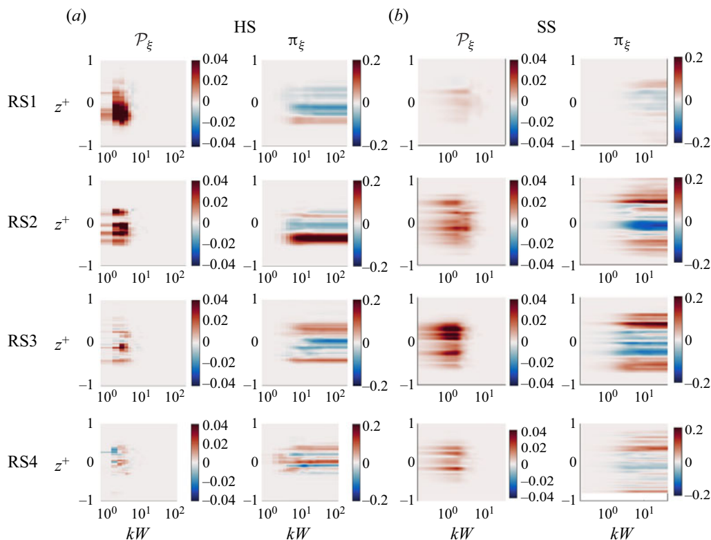
Figure 9. Comparison of the production and transport flux between HS and SS experiments at comparable experiment times.
