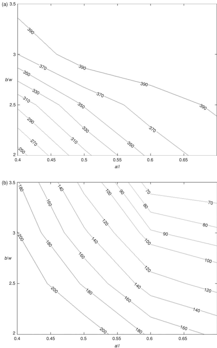
Figure 2.7 The T-match structure matching chart for the case of l = \lambda/2 , w = \lambda/100 , w' = w/2 , (a) resistance ( \Omega ) (b) reactance ( \Omega ).
