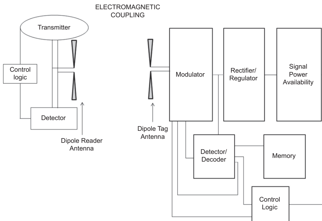
Figure 2.5 Passive tag with electromagnetic back-scattering.
