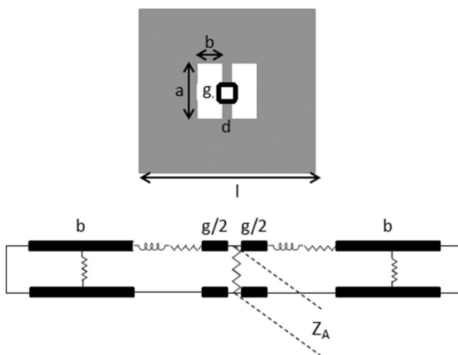
Figure 2.10 The nested-slot structure and the equivalent circuit.
