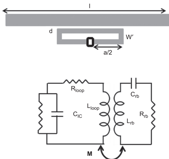
Figure 2.8 Layout of inductively coupled field and equivalent circuit.
