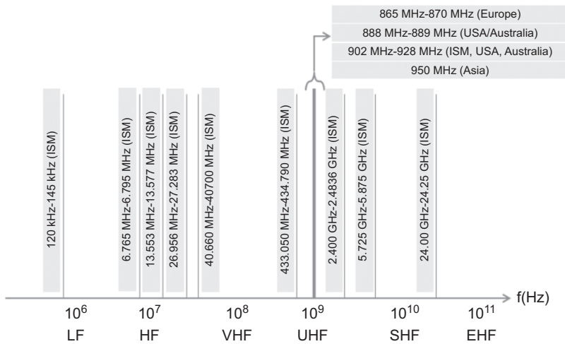
Figure 2.2 Available worldwide frequency bands for RFID.
