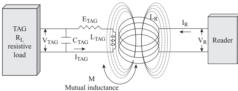
Figure 2.3 Resonant frequency in tags with inductive coupling.
