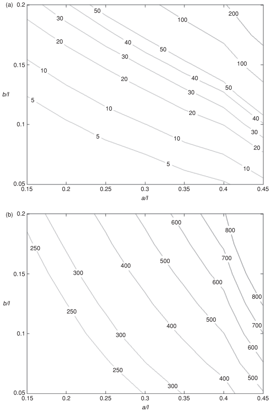
Figure 2.11 The nested-slot structure matching chart for the case of l = \lambda/2 , d = g = \lambda/120 , (a) resistance ( \Omega ) (b) reactance ( \Omega ).
