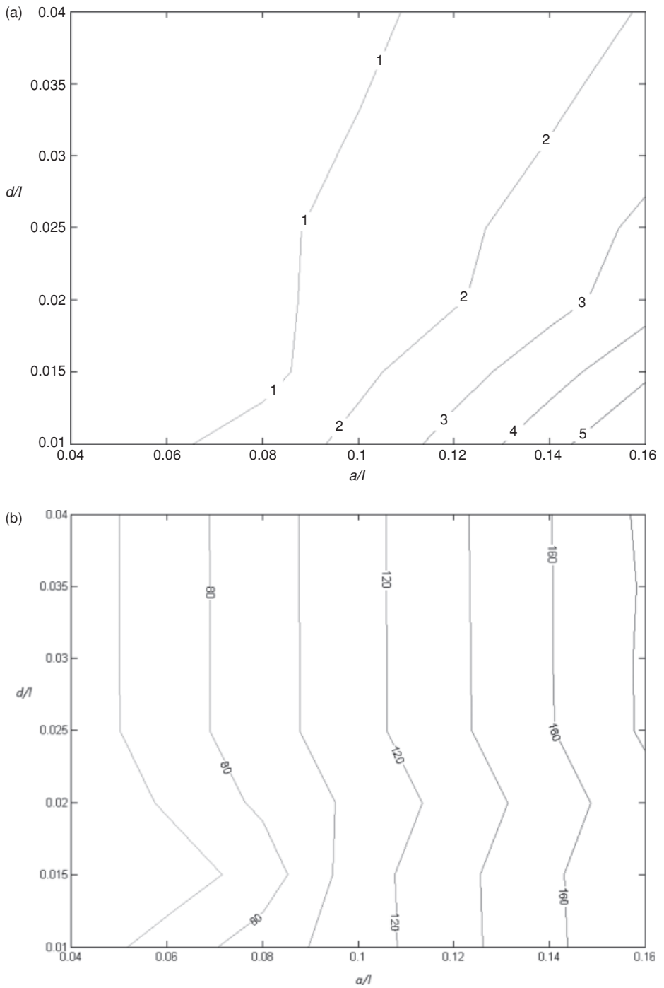
Figure 2.9 The inductive-coupled structure matching chart for the case of a = b , l = \lambda/2 , w = \lambda/100 , w' = w/2 : (a) resistance ( \Omega ) (b) reactance ( \Omega ).
