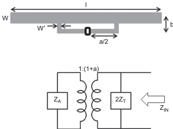
Figure 2.6 The T-match structure and the equivalent circuit.
