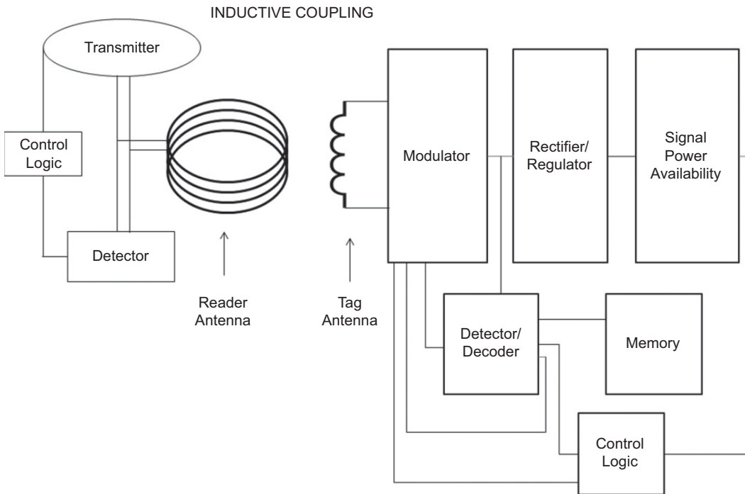
Figure 2.4 Passive tag with inductive coupling.
