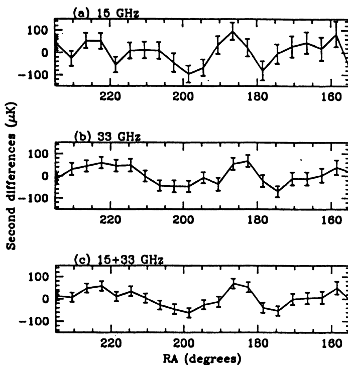
Figure 2. The stacked data scans at Dec= +40^\circ and their one-sigma error-bars in a 4^\circ bin in RA at (a) 15 GHz, (b) 33 GHz and (c) (15+33) GHz.
