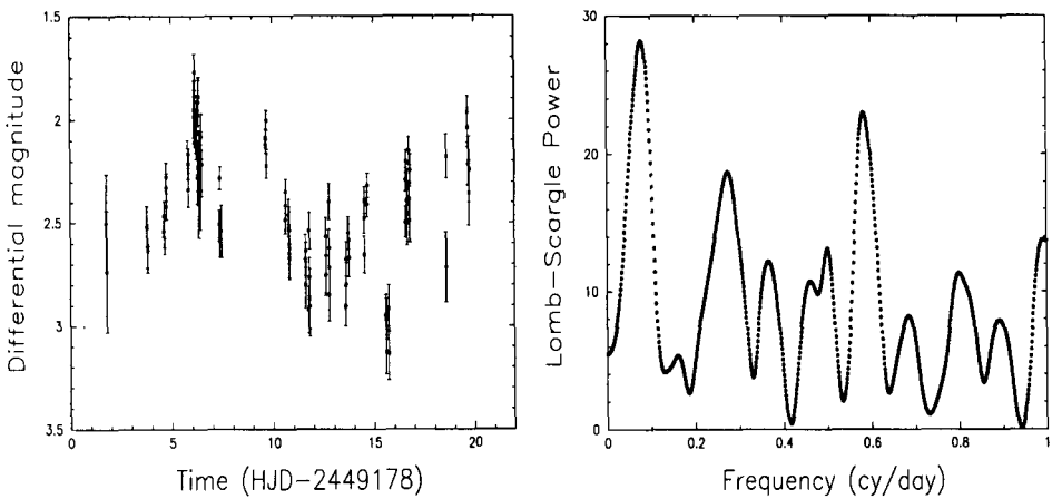
Figure 2. Light curve of star 101 in Fig. 1. Figure 3. Lomb-Scargle statistics power spectrum of the light curve in Fig. 2. Magnitudes in units of average magnitude of comparison stars.
