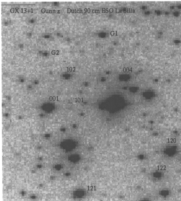
Figure 1. Gunn z band image of GX 13+1. Star 101 is the IR counterpart.
