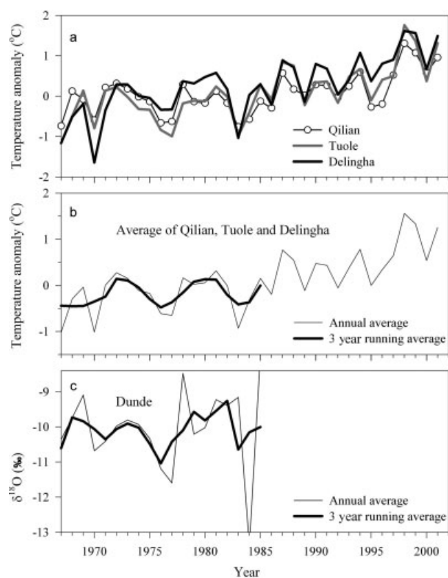
Fig. 6. Air temperatures at three meteorological stations (Qilian, Tuole and Delingha) on the northern TP (a) averaged (b) and compared with the Dunde ice-core \delta^{18}\text{O} record (c).
