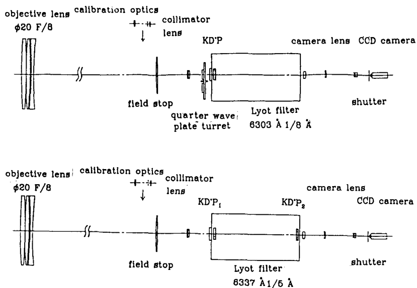
Fig. 1. Optics layout of the Flare Telescope for the measurements of magnetic (upper) and velocity (lower) fields.
