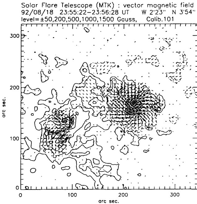
Fig. 2. Vector magnetic field obtained on August 18, 1992. The north is at the top and the east is to the left.
