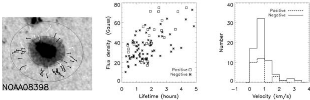
Figure 1. left: An illustration of all the tracks of the unipolar MMFs that we have identified in AR 08398. White arrows represent positive MMFs and black for negative ones, all superposed upon a MDI filtergram. The smaller and larger ellipses are the approximations of the inner and outer boundaries of the moat. middle: a plot of flux densities of selected MMFs in both ARs versus their lifetimes. right: a histogram of the velocities of MMFs in both ARs.
