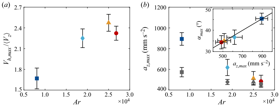
Figure 8. (a) Plot of the non-dimensional maximum horizontal speed in a swing V_{h,max}/\langle V_z \rangle . (b) Behaviour of the maximum vertical acceleration a_{z,max} . The grey symbols represent the descending pendulum model introduced in § 2.3. Inset shows \alpha_{max} versus a_{z,max} together with the best-fit line: \alpha_{max} = (0.03 \pm 0.01)a_{z,max} + (20.8 \pm 6.8) .
