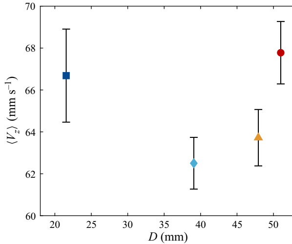
Figure 5. The mean settling velocities ( V_z ) of the particles. Unless further specified, the definitions of the data markers follow table 1 and vertical error bars represent the standard deviation of the measurements.
