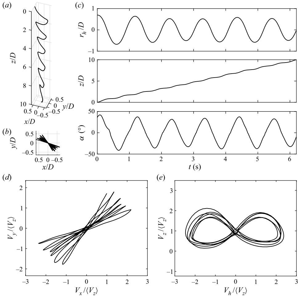
Figure 4. Descent of particle no. 2 ( \theta = 73^\circ , D = 39 mm) after removing transient motions and dedrifting. (a) Three-dimensional and (b) top view of the trajectory reconstruction. (c) (From top to bottom) The radial displacement along the direction of motion r_h , the depth z and the pitch angle \alpha plotted against time t . No rolling motions are observed. (d) Velocity in the y -direction V_y plotted against that in the x -direction V_x . (e) Instantaneous vertical velocity V_z against the horizontal velocity V_h = \pm(V_x^2 + V_y^2)^{1/2} whose sign switches every swing. All velocities and positions are normalised with the mean descent velocity \langle V_z \rangle and diagonal length D of the particle, respectively.
