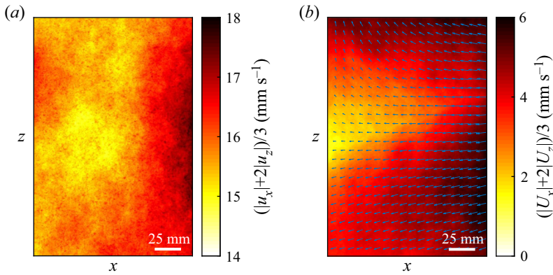
Figure 17. The PIV measurements of the flow in the turbulence box. The time-averaged (a) r.m.s. flow velocity fluctuation field and (b) mean flow field at the middle of the tank. The subscripts ( x, z ) denote the corresponding velocity components.
