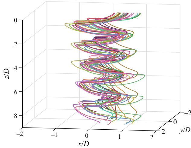
Figure 3. Reconstructed three-dimensional trajectories of particle no. 2 ( \theta = 73^\circ , D = 39 mm) in quiescent fluid.
