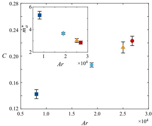
Figure 10. Fitting parameter C as a function of Ar . In the context of underwater pendulums, C is related to the added-mass coefficient m_a^* . Inset shows m_a^* versus Ar .
