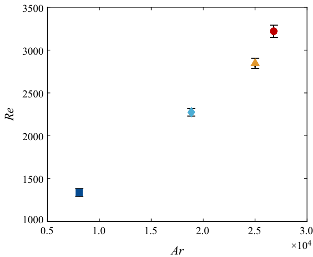
Figure 6. Plot of Re against Ar . A linear relation is observed for the first three points and a kink seen for the last, which suggests a transition in settling style. As Re(Ar) is one-to-one in the investigated range, the two are used interchangeably.
