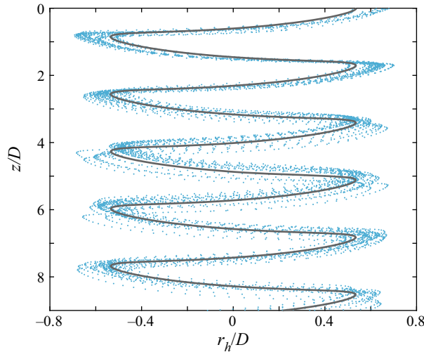
Figure 9. Model pendulum trajectory (grey line) overlaid on the experimental data of particle no. 2.
