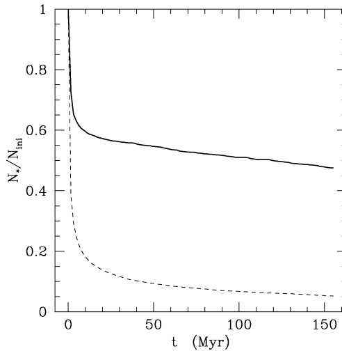
Figure 3. Evolution of the fraction of first- (dashed line) and second-generation (full line) stars still bound to the cluster with initial parameters: SFE of 0.33, r_h/r_t = 0.06 and \tau_M/t_{\text{cross}} = 0.33 .
