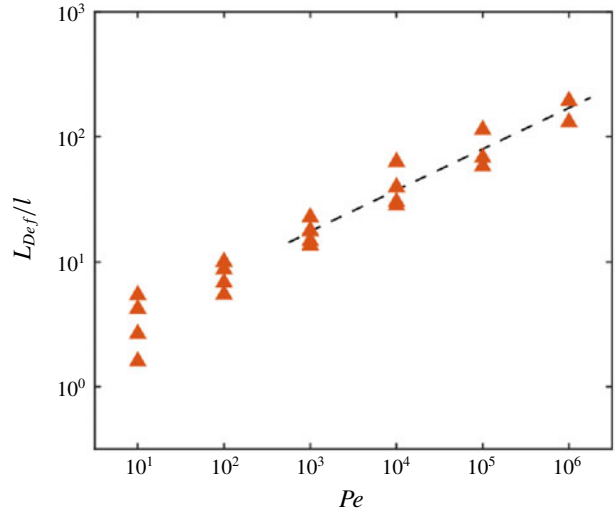
FIGURE 9. Simulated Pe versus L_{Def}/l for 10^{-2} \leq Re < 10^2 and no buoyancy forces. The dashed line is Pe^{1/3} . Simulations in which L_{Def} did not reach steady state are not included. The Re = 10^2 case is addressed in the next section.
