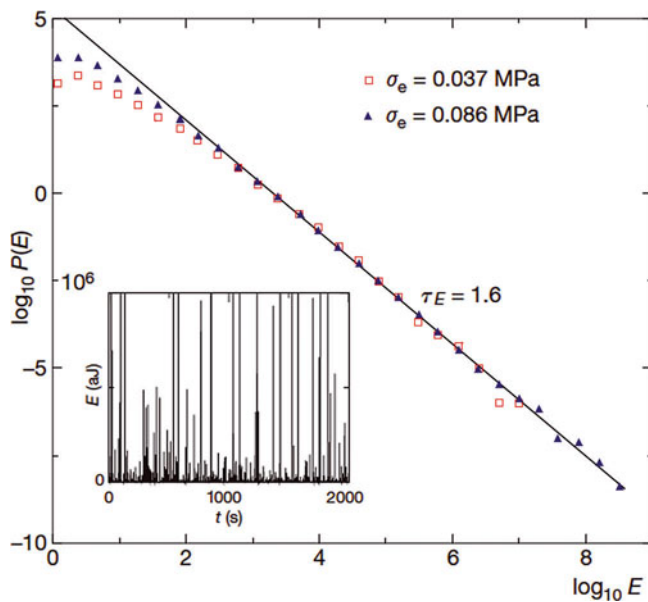
Fig. 4. Distribution of acoustic energy bursts recorded in ice single crystals under creep tests at -10^{\circ}\text{C} . Inset is a typical recorded acoustic signal (from Miguel and others, 2001). Nature by Nature Publishing Group. Reproduced with permission of Nature Publishing Group via Copyright Clearance Center.
