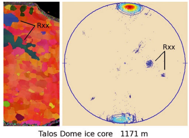
Fig. 7. Fabric of an ice sample from the Talos Dome ice core; Rxx shows the correspondence between the ice texture and fabric for two grains. Talos Dome is on the edge of the East Antarctic plateau (72°47'S, 159°04'E; 2318 m a.s.l.); a 1620 m ice core was recovered in 2007 (Urbini and others, 2008).
