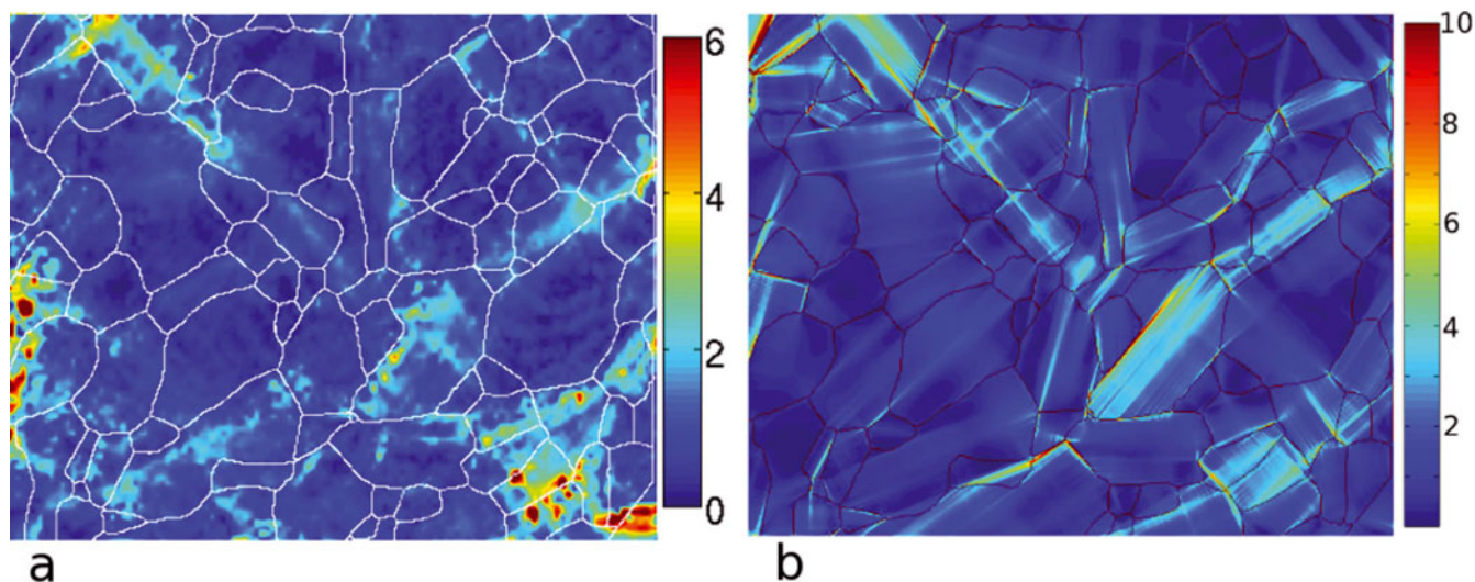
Fig. 9. Comparison between (a) measured equivalent strain field in columnar ice and (b) simulated strain-rate field using the full-field viscoplastic FFT approach. In both cases, values are normalized by the average.
